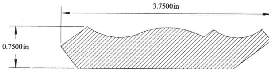
CR-3750 \frac{3}{4} " x 3\frac{3}{4} " Crown
