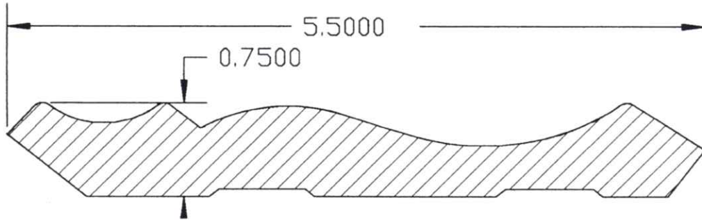
CR-5500 \frac{3}{4} " x 5\frac{1}{2} " Crown
