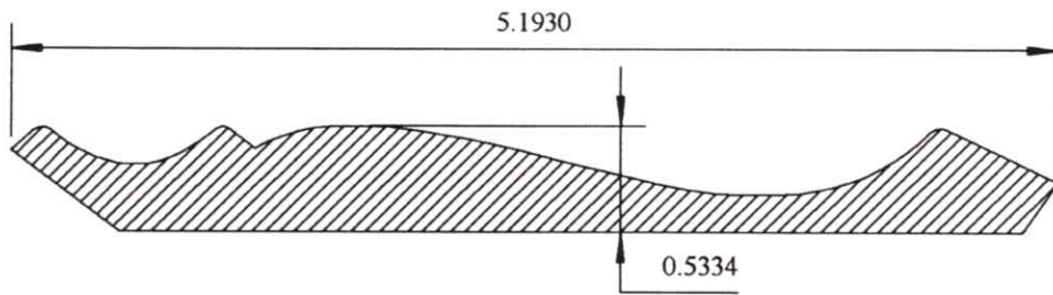
CR-5193 \frac{1}{2} " x 5\frac{3}{16} " Crown (Oster)
